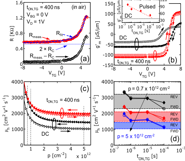
Fig. 5. (a) Hole R - V_{TG} measured ( R_{\text{meas}} ), fitted ( R_{\text{fit}} ) as in [35], and with contact resistance ( R_C ) subtracted ( R_{\text{meas}} - R_C ). (b) Intrinsic transconductance ( g'_m ) from Fig. 3(b), as a function of V_{TG} from pulsed (red) ( t_{\text{ON},TG} = 400 ns) and dc (black) measurements. Arrows indicate direction (FWD or REV) of sweep. Inset shows maximum |g'_m| (from FWD sweeps) as a function of gate ON-times. (c) Extracted hole mobility as a function of carrier density ( p ) from Fig. 5(b). (d) Hole mobility versus t_{\text{ON},TG} for different p = 0.7 (black), 1 (red), and 5 \times 10^{12} \text{ cm}^{-2} (blue). Values extracted from Fig. 5(c) at the marked (vertical dashed lines) concentrations. Open circles and solid diamonds are from FWD and REV pulsed sweeps, respectively. Values extracted from dc FWD and REV sweeps mark limits of shaded regions. Note large mobility uncertainty of dc sweeps (up to \sim 1000 \text{ cm}^2 \text{ V}^{-1} \text{ s}^{-1} or \sim 30\% ) compared with pulsed sweeps ( \sim 50 \text{ cm}^2 \text{ V}^{-1} \text{ s}^{-1} or \sim 2\% ).
