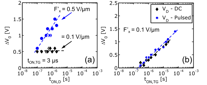
Fig. 6. (a) Dirac voltage shift ( \Delta V_0 ) as a function of drain ON-time ( t_{\text{ON},D} = 100 \text{ ns} - 2 \mu\text{s} and t_{\text{ON},TG} = 3 \mu\text{s} ). The V_{TG} sweeps (not shown) are from -8 to 8 V and back to -8 V, while V_D is increased from 1 (black diamonds) to 3 V (blue circles). V_D values correspond to intrinsic lateral fields F'_x \approx 0.1 and 0.5 \text{ V}/\mu\text{m} , respectively, after contact resistance is subtracted ( L \times W = 3 \times 9 \mu\text{m} ). (b) \Delta V_0 versus t_{\text{ON},TG} (300 ns–80 \mu\text{s} ). The drain terminal is biased using a dc (diamonds) and pulsed bias (circles) ( F'_x = 0.1 \text{ V}/\mu\text{m} and t_{\text{ON},D} = 0.5 \cdot t_{\text{ON},TG} ).
