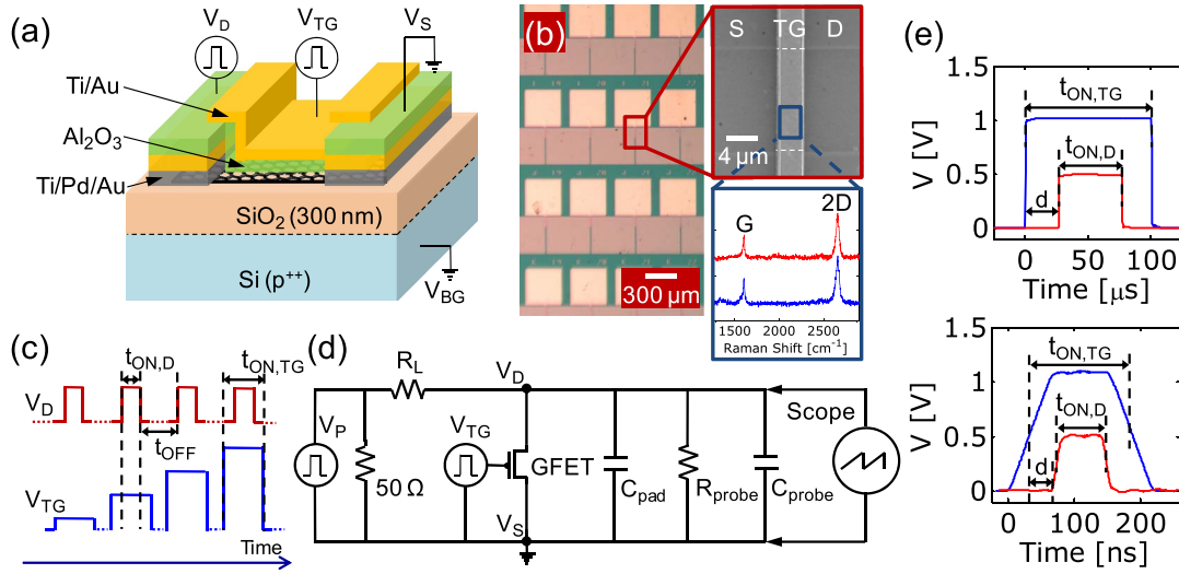
Fig. 1. (a) Schematic diagram of top-gated GFETs fabricated in this paper. (b) Optical and SEM images as well as Raman spectra of typical devices. (c) Schematic diagram of pulses and biases applied at top-gate ( V_{TG} ) and drain ( V_D ) terminals. The amplitude of V_{TG} is increased when performing a gate sweep of the voltage. (d) Diagram of a circuit used to apply voltage pulses at drain and gate terminals. Current is calculated from the voltage drops across the load resistor ( R_L = 0.5 - 1.5 \text{ k}\Omega ), GFET, probe resistance ( R_{probe} = 100 \text{ k}\Omega ), and pad ( C_{pad} = 8.3 \text{ pF} ) and probe capacitances ( C_{probe} = 0.8 \text{ pF} ). (e) Measured drain and top-gate pulses—top gate scope connection not shown in (d)—with t_{ON,TG} = 100 \text{ }\mu\text{s} and t_{ON,D} = 50 \text{ }\mu\text{s} (top) and t_{ON,TG} = 150 \text{ ns} and t_{ON,D} = 75 \text{ ns} (bottom). In both cases, V_D has a delay d = t_{ON,D}/2 relative to V_{TG} . In addition, V_{TG} = 1 \text{ V} and V_D = 0.5 \text{ V} .
